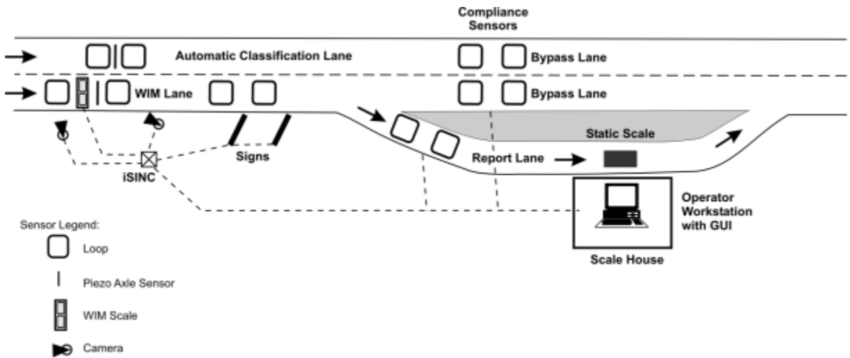
Figure 2 – Typical NB/NS Weigh Station Sorting System Layout
